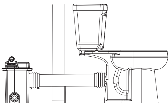
BEHIND THE WALL INSTALLATION (Use Extension Kit p/n 10-3050)
