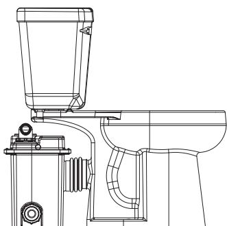
STAND-ALONE INSTALLATION
